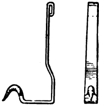
Fig. 148.—Climbing-irons. (After Boppe.)
